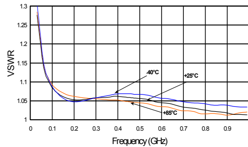
VSWR, 1000 pF
