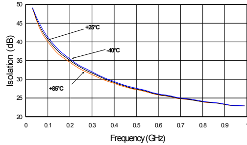
Isolation, 1000 pF
